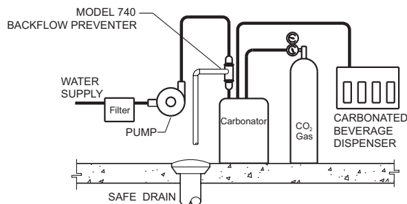
Carbonated Beverage System
