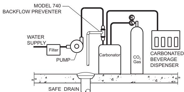
Non-Carbonated Beverage System
